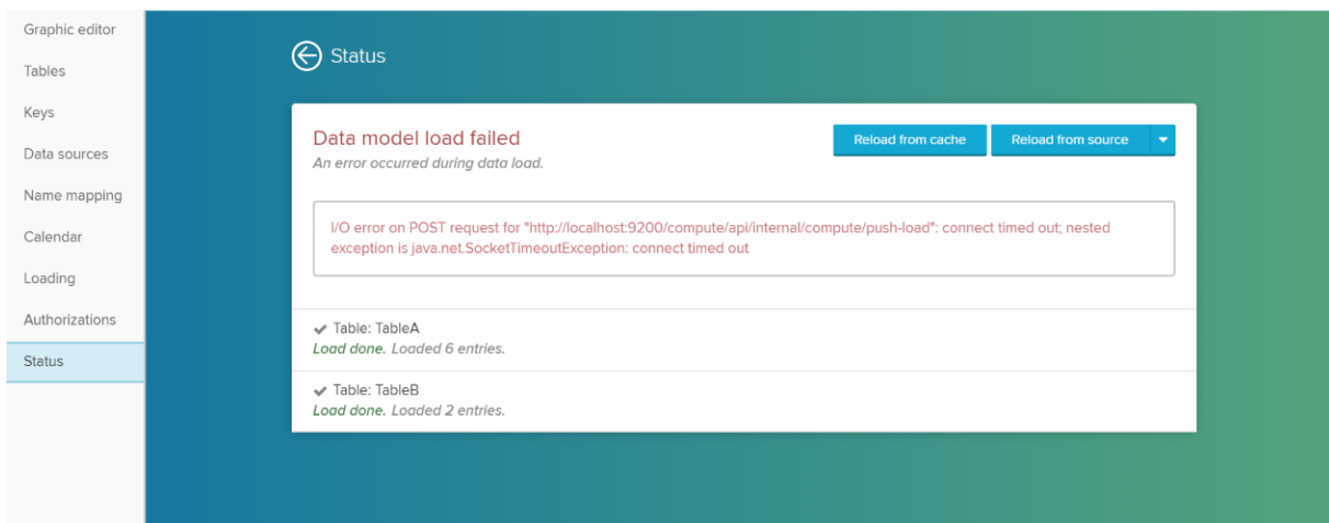
Figure 8: The compute service on port 9200 has not been started
